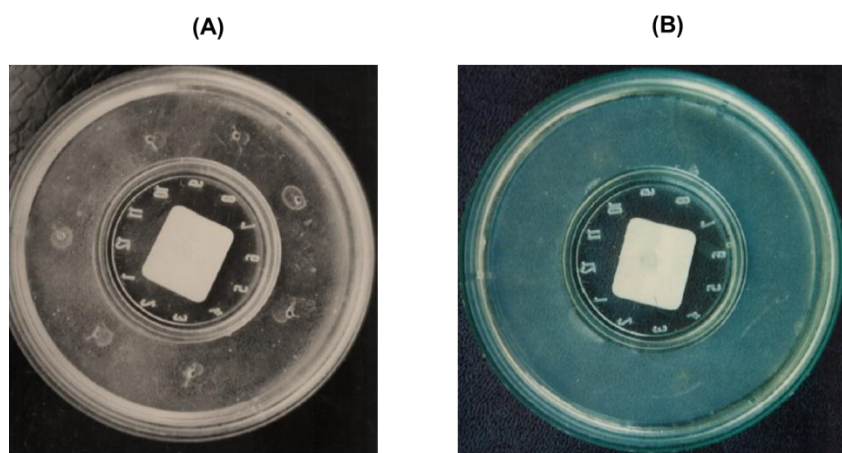
Fig. 4: Antigen-antibody reaction of the insoluble complex by Ouchterlony double diffusion,
