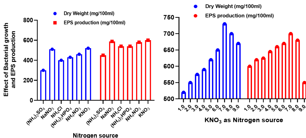
Fig. 1: Effect of the nitrogen source (A) and the \text{KNO}_3 level on growth and EPS production by A. tumefaciens
