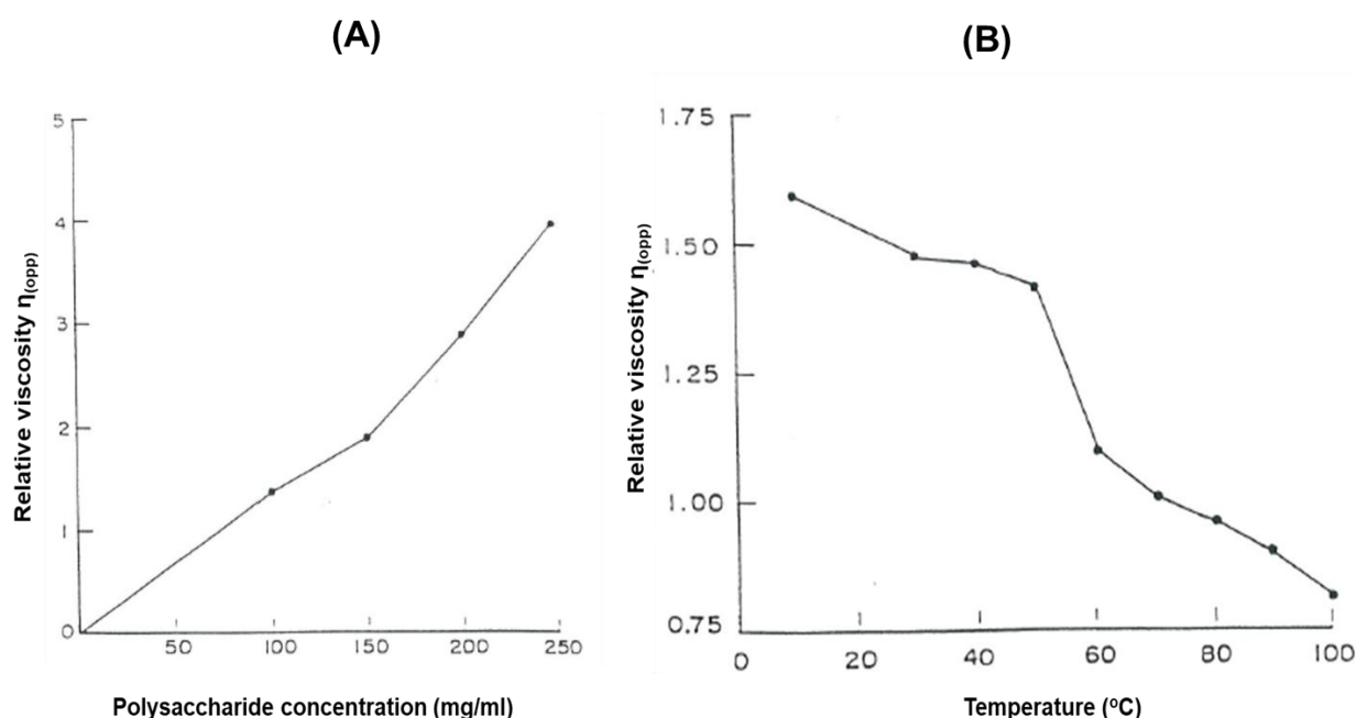
Fig. 3: Estimation of relative viscosity (RV) (A) and effect of temperature on RV of the purified EPS (B)
