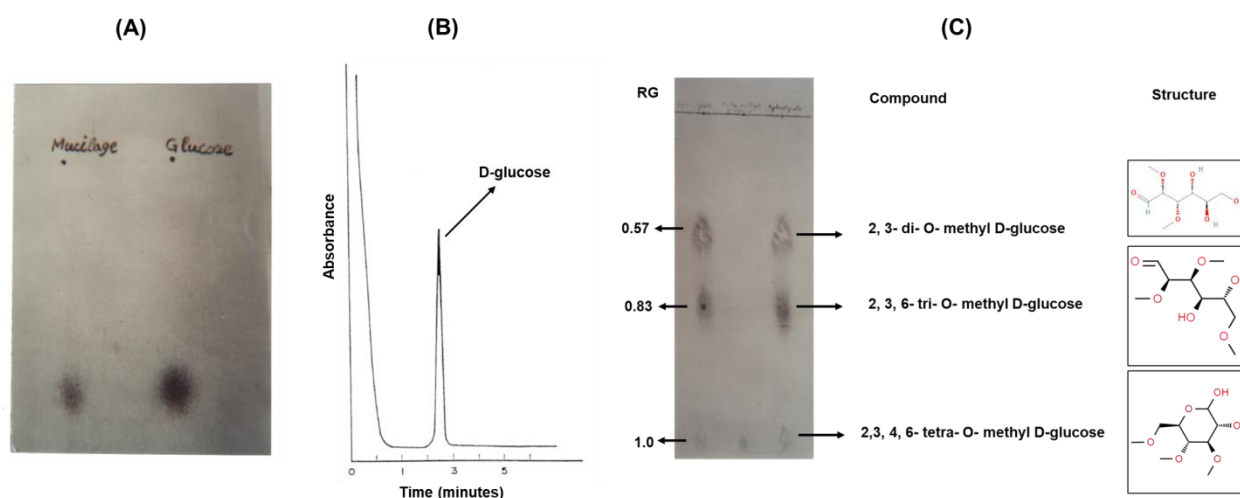
Fig. 2: Paper chromatogram of the sugar components (A), acid hydrolysate of purified EPS (B) and methylation (C) of EPS produced by A. tumefaciens
